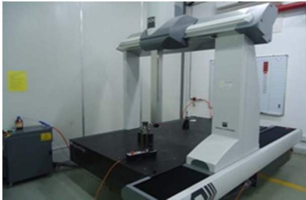
3D-measuring machine HEXAGON GLOBAL ADVANTAGE PCDIMS+ QUINDOS To check gears and complicated structures of parts
