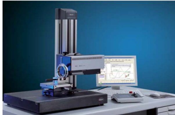
Profile Meter MAHR Surf XC 20 To check profile of pin, roller and pinion shaft and others parts
